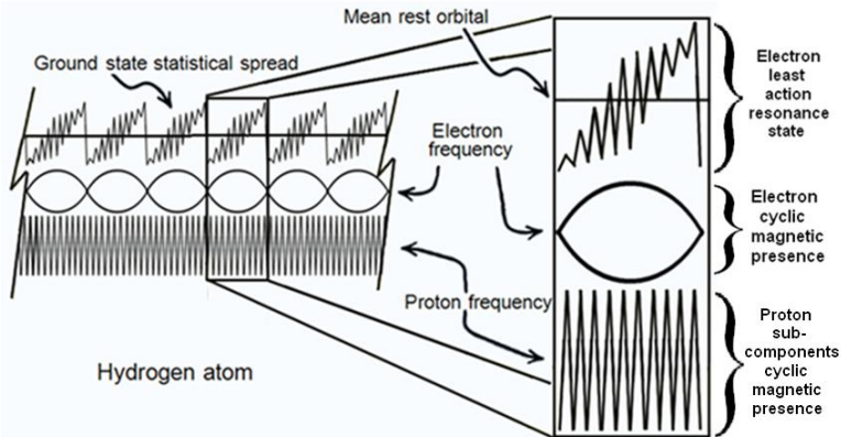
Figure 3: Establishment of the least action resonance state of the electron in the hydrogen atom.
