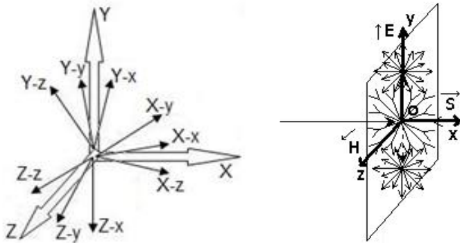
Figure 1: The orthogonal structure of the 3-spaces geometry complex, and plane wave reference frame applied to a permanently localized photon.
