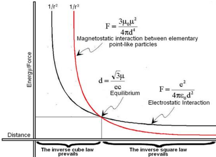
Figure 2: Intersecting inverse square and inverse cube interaction curves.
