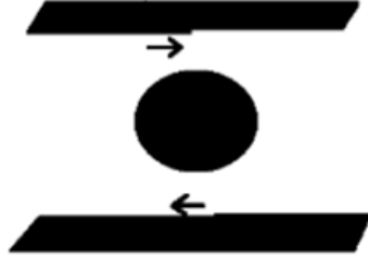
Figure 2: Longitudinal bi-directional energy flow proportional to transverse wave moving at c . This is dark energy.
