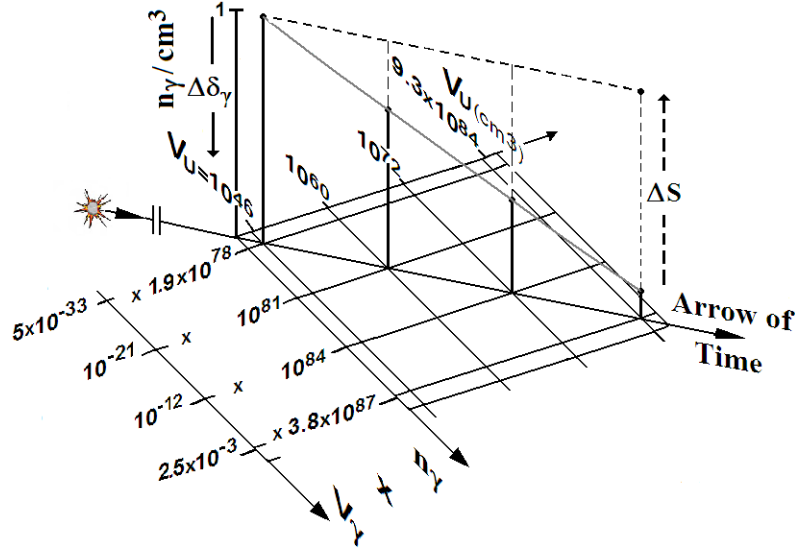
Fig. 4: Increment of CMB system entropy ( \Delta S_{CMB} ). The chronology of CMB density ( \Delta\delta_\gamma: n_\gamma/cm^3 ), was used to plot normalized the entropy change from the Era of equal number of photons and baryons to present, \Delta S_{CMB[n_\gamma=nB/prs]} . The latter, is illustrated by vertical lines, which integrate the decreasing enthalpy ( \Delta H : full lines) with its corresponding entropy increase ( \Delta S : broken lines). The cosmos volume increases from 1.5 \times 10^{48} \text{ cm}^3 to 9.3 \times 10^{84} \text{ cm}^3 . Photon density decreases according to a geometric progression 1.25 \times 10^{-1} . The c appears to indicate the presence of a space-time restriction to expansion. As described: V_{\gamma-RELIC-CMB} = 2.5 \times 10^{-3} \text{ cm}^3 \times n_{\gamma prt} = \text{total } V_{U-RELIC-CMB} or V_{U-prt} = 9.3 \times 10^{84} \text{ cm}^3 .
