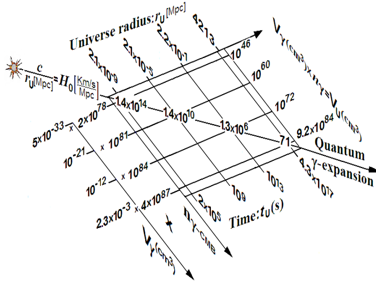
Fig.1: Observation vs. calculated Quantum Integrated Expansion. The figure, shows that the multiplication: n\gamma \times V\gamma [ cm^3 ] = V_U [ cm^3 ], determines the quantum-integrated volume of the universe in cm^3 , under the relativistic restriction: radius of the universe in cm over its elapsed time in seconds: r_U [cm]/ t_U [s] = c [cm/s]. If the chronological radius of the universe equals recession distance: r_U = \bar{r} . The velocity of expansion could be measure, after the appearance of galaxies, as a recession velocity: \bar{v} = \bar{r} [Mpc] \times H_0 \therefore r_U [Mpc] \times H_0 [km/s/Mpc] = c , as shown in the figure: c [km/s]/ \bar{r}_U [Mpc] = H_0 [km/s/Mpc]. Hence, r_U = t_U \times c \therefore t_U \times c \times H_0 = c \Rightarrow H_0 = 1/t_U = 3.086 \times 10^{19} \text{ km} / t_U \text{ /Mpc, } t_U [s], example: H_0 = 3.086 \times 10^{19} \text{ km} / 4.34 \times 10^{17} \text{ s /Mpc} = 71.1 \text{ km/s/Mpc} .
