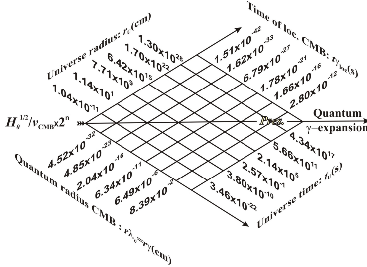
Fig.2: Plotting merging quantum and relativistic parameters. The quantum dimensions starting as: r_{\gamma_{pl}} / t_{\gamma_{pl}} = c , are quantum dimensions which interrelate with c a relativistic parameter. The photon radius r_{\gamma} as 4/3 \times \pi \times (r_{\gamma})^3 adds to the observable universe volume dimensions, t_{\gamma_{loc}} does not, but c links universe radius as a function of the universe time. Total energy ( E_T = \text{entropy} + \text{enthalpy} ) for its conservation at the level of CMB, requires a compensatory mechanism like the spontaneous PdC-process, in which the halving of the energy of 1 photon generates 2 of twice the original- \lambda and conservation of momentum. Accordingly, even if photons are subject to Gravity, a dynamic CMB structured-vacuum could expand by a PdC-dependent \Delta n_{\gamma} and \Delta V_{\gamma} a process independent of Gravity.
