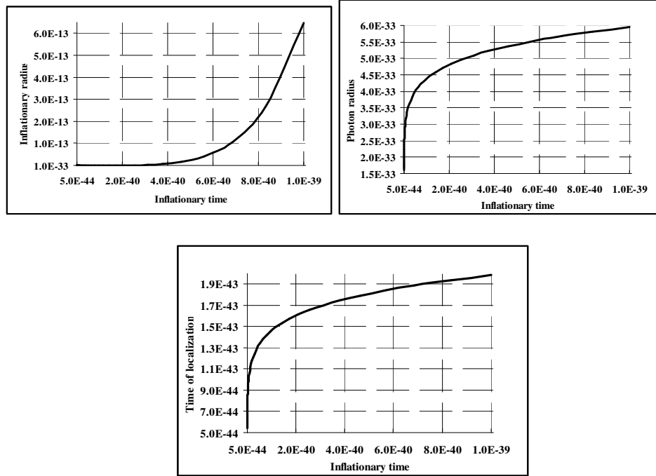
Fig.3: Inflation. Illustrate that the total energy E_T (or critical energy E_c ) becomes quantized in the course of inflation as Planck (Pl) particles each one generating by PdC two photons of half energy. Thus, expanding by 2 \times 8 = 16 the space-time locus, allowing a chain reaction of additional Planck photons incoming into the inflationary universe, up to summa of their energy equals E_T .
