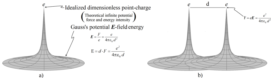
Figure 10: Test point-charge and potential E-field representation as conceptualized by Gauss, and theoretical point-charges interaction as initially established by Coulomb.
