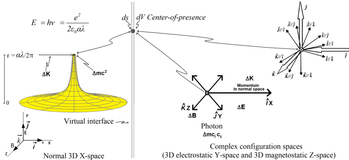
Figure 17: Idealized representation in the trispatial geometry of an electromagnetic photon \Delta K momentum energy related to half of its energy quantum residing in X-space and of the stable stationary oscillation of the other half of its energy between configuration spaces Y and Z.
