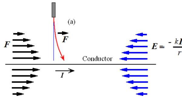
Figure 4. Possible parallel electric field being produced by a straight long current.
