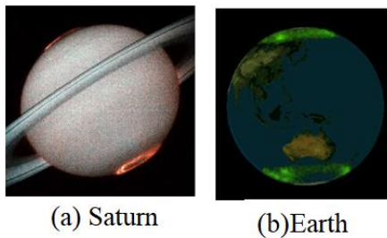
Figure 12. Aurora produced at the poles of planets in the form of rings.
