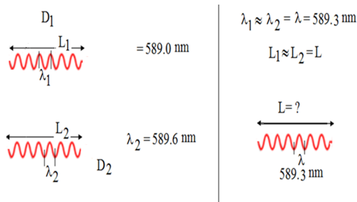
Fig. 3. Sodium atom emits two wavelengths - \lambda_1 and \lambda_2 which are very close.
