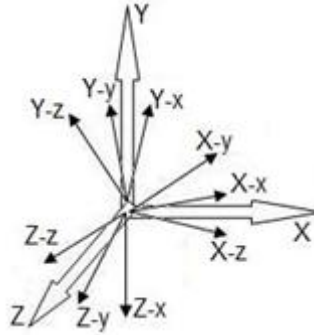
Fig.1: Orthogonal structure of the 3-spaces model.
