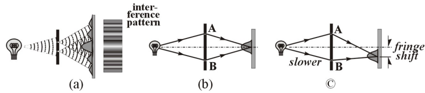
Fig. 27. Double-slit experiment.
