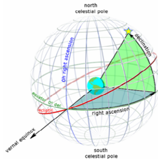
Fig. 0-25. Celestial coordinates 128 .
