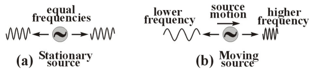
Fig. 0-16. Doppler effect (1).
