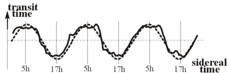
Fig. 0-14. deWitte's results.
