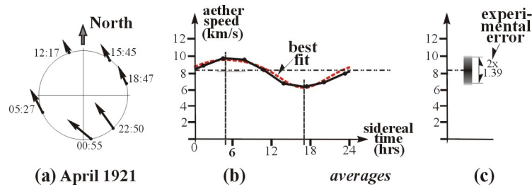
Fig. 12. Miller's results 53 .
