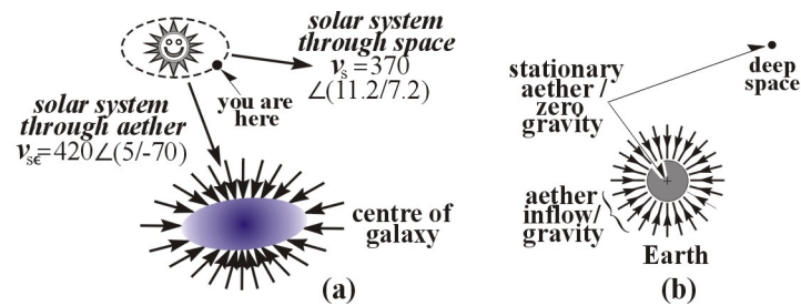
Fig. 19. Aether: absolute speeds; gravity a .
