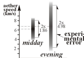
Fig. 0-9. Michelson-Morley results.
