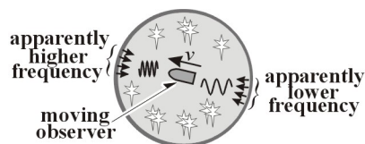
Fig. 18. Microwave background.
