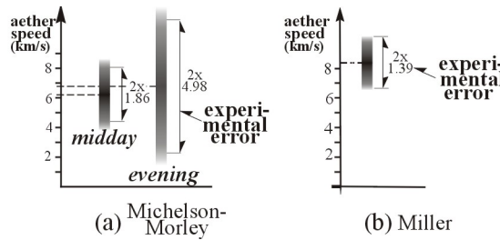
Fig. 0-23. Michelson-Morley. Miller results.
