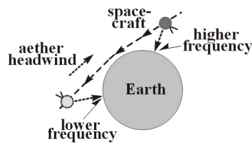
Fig. 0-15. Spacecraft flyby.
