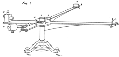
Fig. 7. Michelson's 1881 interferometer 29 .
