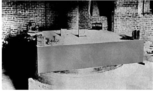
Fig. 8. Michelson's 1887 interferometer 33 .
