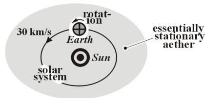
Fig. 0-5. Earth's orbit.
