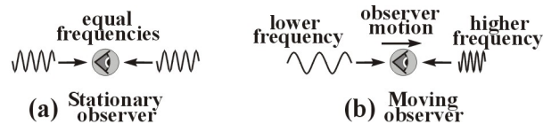
Fig. 0-17. Doppler effect (2).
