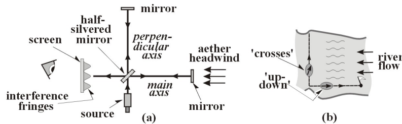
Fig. 6. Michelson-Morley (1).
