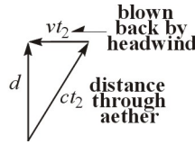
Fig. 0-28. Interferometer, p-axis{{interfer}}.
