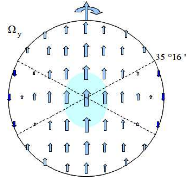
Figure 3.a. Vector topology of the gyrotation along the spin axis of a spinning sphere. The spin axis contains the highest amplitude of gyrotation. At the latitude of 35^\circ 16' , the gyrotation becomes zero. At the equator, gyrotation is inverted, and one gets a local increase of the global attraction!
