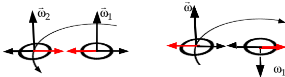
Figure 1.a. Like-oriented elementary particles of trapped 'light', hit by an orbiting graviton and undergoing a Coriolis acceleration \vec{a}_C . The impact deviates the graviton (small black arrows). The particles attract reciprocally due to Newton's third law (red arrows).
