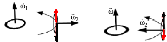
Figure 2.a. and b. Elementary particles of trapped 'light' under a right angle, hit by an orbiting graviton and undergoing a Coriolis acceleration \vec{a}_C . One particle accelerates tangentially. The impact deviates the graviton (small black arrows). The particles attract reciprocally due to Newton's third law (red arrows). Remark that there is no reciprocity.
