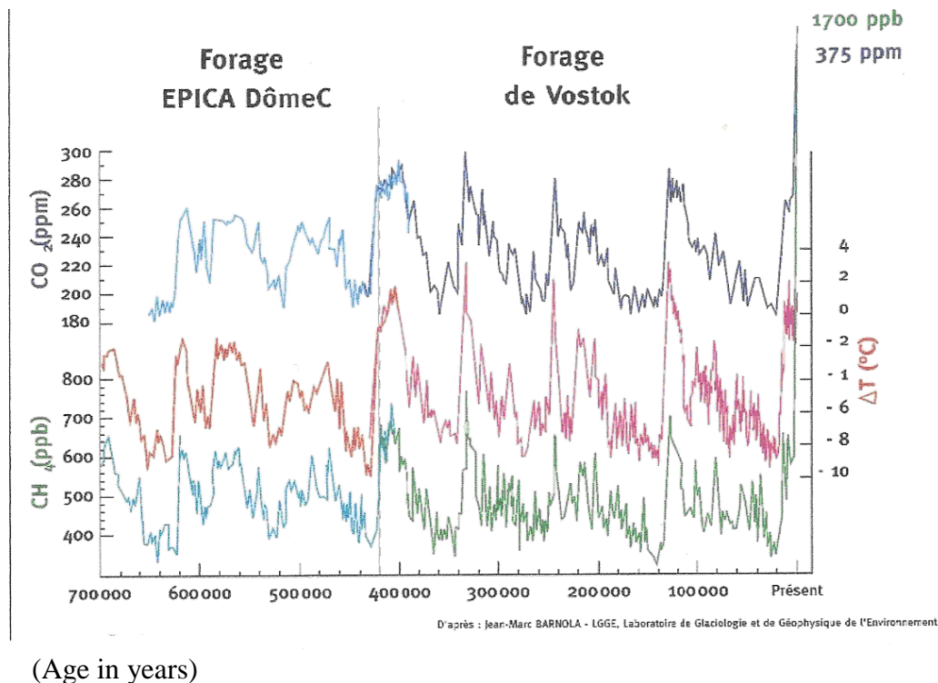
Figure 1. The concentration of atmospheric CO 2 (upper curve) and CH 4 (lower curve) with the variations of temperature (central curve) for the last 700 000 years.
