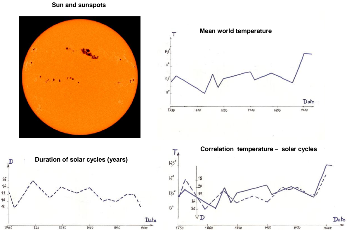
Figure 4. A) The Sun with its spots. B) The mean Earth temperature from 1750 to 2000. C) The duration of solar cycles in the same interval. D) The correlation between the two phenomena (The scale of duration has been reversed in order to emphasize the correlation).
