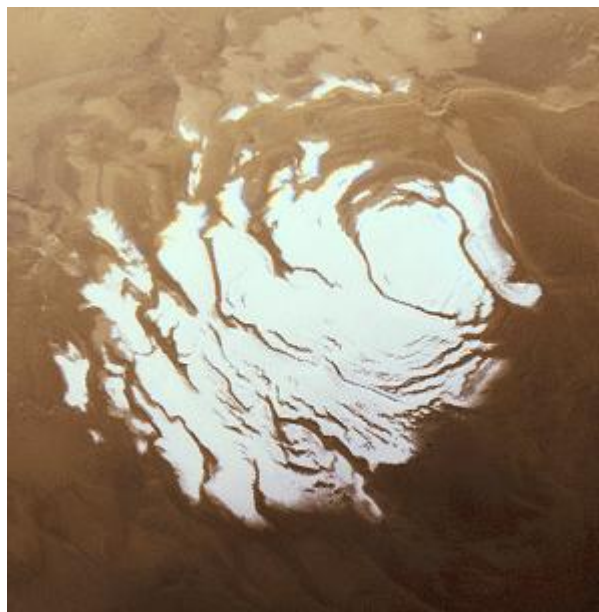
Figure 2 A recent picture of the Martian south polar cap.
