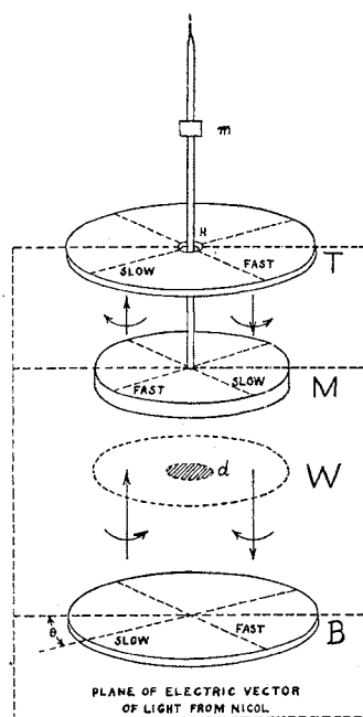
FIG. 3. Wave plate arrangement.
