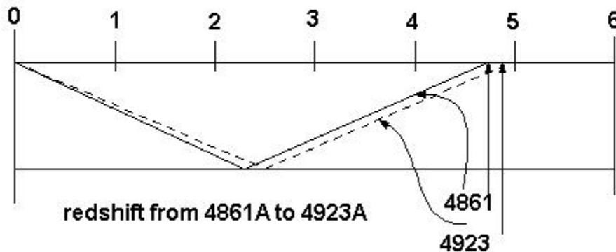
Figure-1 illustrating a wavelength of 4861 0 red shifted to 4923 0 , a marginal difference of 62 0 .
