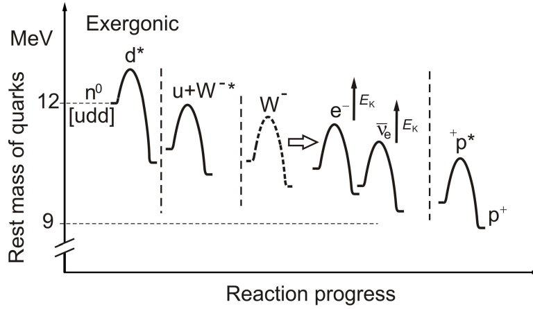
Figure 3. Illustrates the intermediate reaction d \rightarrow u + W^- \rightarrow u + e^- + \bar{\nu}_e . The transition states involves the reactions of one quark u plus boson W^- which decays in products: proton, electron and antineutrino. W^- confers transition energy (activation) and asymmetry. A dotted curve indicates a much shorter half-life of the transition states which in this context prevents the reversibility of products into substrate. The very short half-life of W^\pm allows that the transition-activation energy dissipate and prevents reaction equilibrium. Symmetry quantity n \leftrightarrow \bar{n} would yield a similar representation of the disintegration of antineutron: \bar{n}^0 \rightarrow p^- + e^+ + \nu_e ( \bar{d} \rightarrow \bar{u} + W^+ \rightarrow \bar{u} + e^+ + \nu_e ) (involve the vector boson W^+ ) and therefore is not illustrated. The scale is based on the resting mass of two down quarks ( d ) of 5 MeV each and one up ( u ) of 2 MeV. (*) Excited or transitions states. The arrow \uparrow indicates that the emission of electrons and antineutrinos escape from the system.
