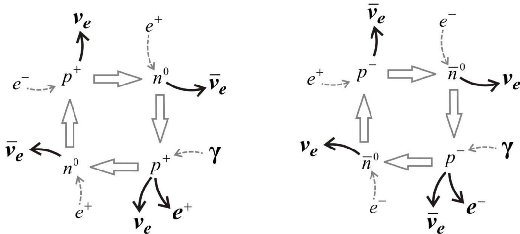
Figure 2. Coupling between reactions allows cycles; this one shows that one electron and one positron are consumed to absorb gamma radiation, generating neutrinos and antineutrinos.
