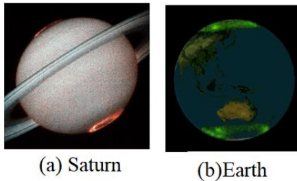
Figure 12. Auroras produced at the poles of planets in the form of rings.
