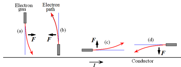
Figure 3. Deflections in CRT in the field of a straight long current.
