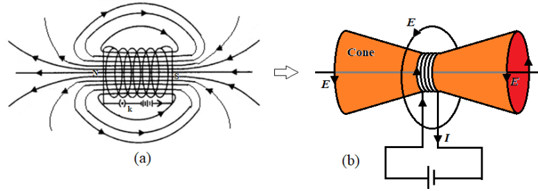
Figure 7. Electric field of a current carrying coil having two electric field cones.
