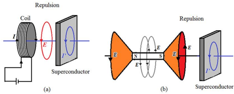
Figure 9. Electric current produced in a superconductor due to (a) electric field of a coil and (b) electric field of a bar magnet.
