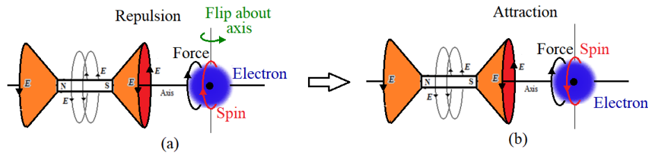
Figure 16. Representation of magnetization produce in magnet material when the spin of an unpaired electron is in same direction of the electric force of the external bar magnet where spin direction gets flipped about vertical axis.
