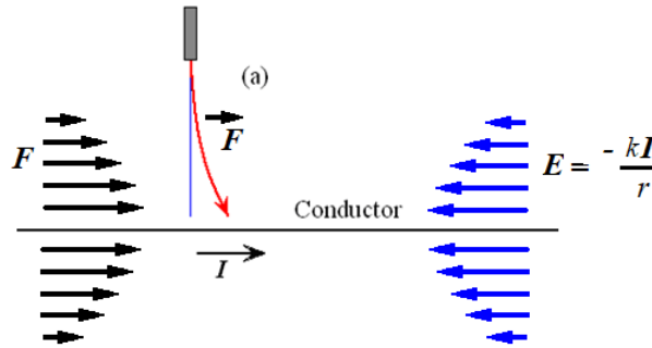
Figure 4. Possible parallel electric field being produced by a straight long current.
