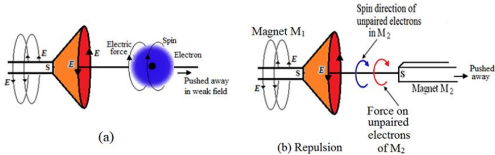
Figure 14. Representation of attraction between two poles of bar magnets.
