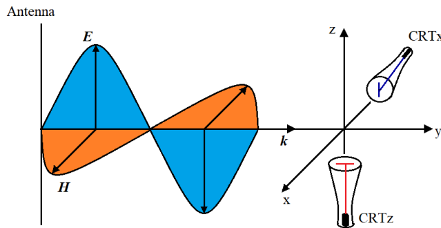
Figure 17. Experimental arrangement to determine change in electric force and magnetic force with frequency on electron beam of CRTs applied by an EM wave produced by an antenna.
