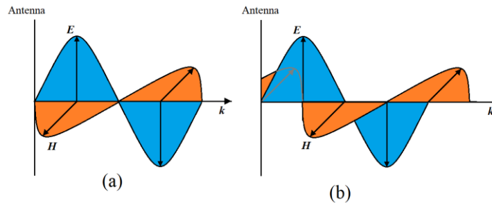
Figure 20. According to the existing classical electrodynamics, phase difference between electric and magnetic field waves in an EM should be zero. (b) According to the expectations from the above experiment, phase difference between electric and magnetic field waves in an EM should be 90 degrees.
