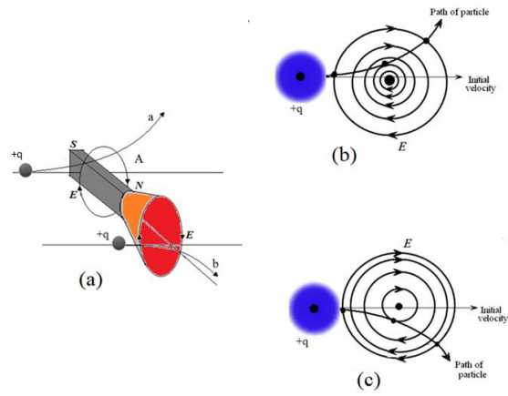
Figure 10. (a) Deflections of a charged particle in the field of a bar magnet. (b) Circular electric field of bar magnet decreasing in magnitude away from center. (c) Circular electric field of bar magnet increasing in magnitude away from center.
