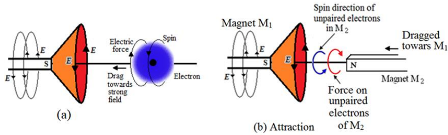
Figure 13. Representation of attraction between two poles of bar magnets.
