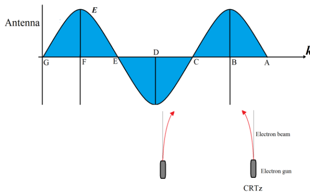
Figure 18. Deflections of electron beam in the asymmetric electric field of EM wave.
