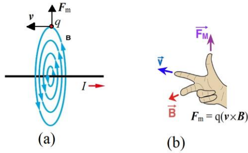
Figure 1. Magnetic field of straight long conductor carrying current and magnetic force on a charged particle.
