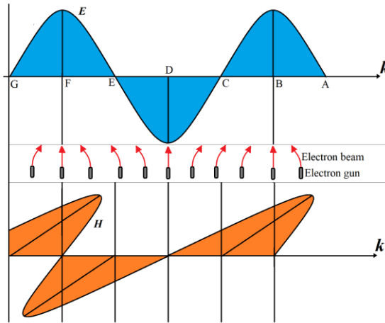
Figure 19. Deflections of electron beam in the asymmetric electric field of EM wave showing a phase difference of 90 degrees in electric and magnetic field waves.
