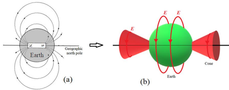
Figure 11. Electric field of earth in absence of solar wind.
