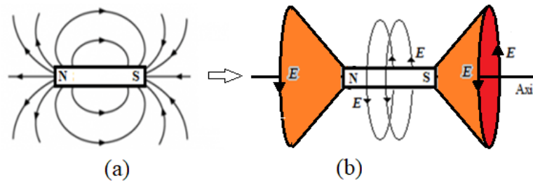
Figure 8. Electric field of a bar magnet having two electric field cones.
