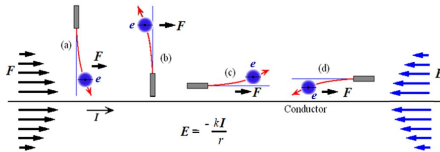
Figure 6. Explanation of deflections of electron beam in different directions using force through field-field interaction in asymmetric electric field.
