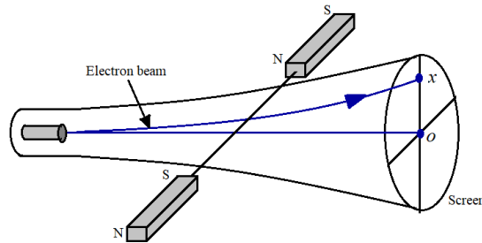
Fig. 8. Deflection of electron beam in e/m by Thomson experiment.
