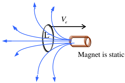
Figure 7 F = qV_q \times B
