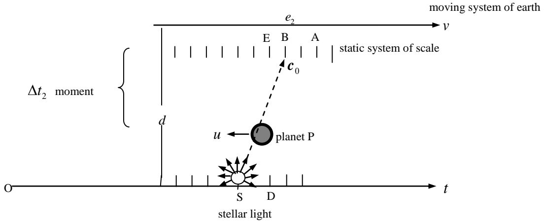
Figure 22 Positions of stellar S, planet P and measurer e in the static system at \Delta t_2
